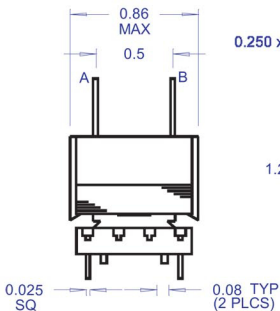
Model 16050 with PCB connections.
