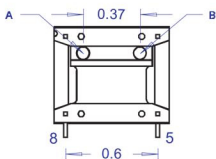
Model 16050 with PCB connections.
